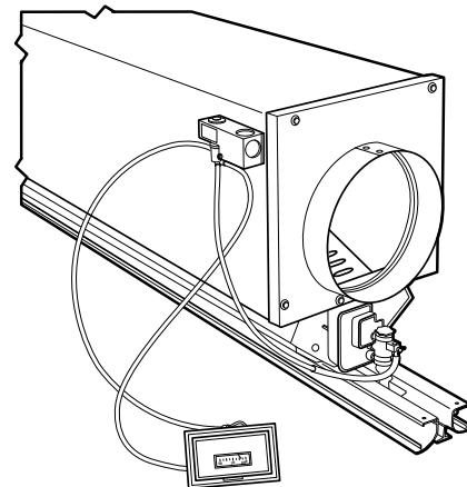
Fig. 50 — VAV Control Arrangement for Electric Changeover
